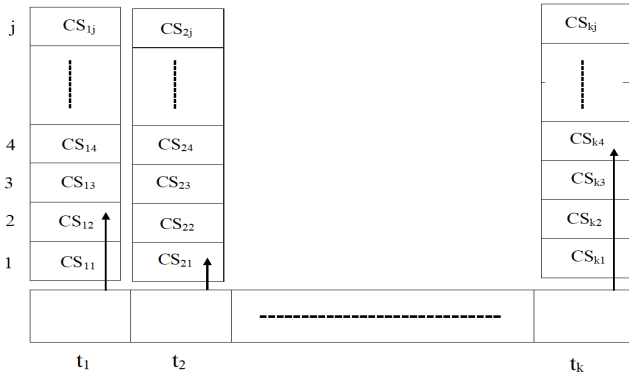
Fig. 3: Chromosome encoding
