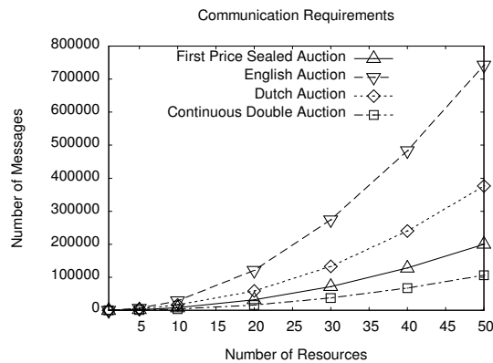
Figure 3. The communication demand of different protocols.
