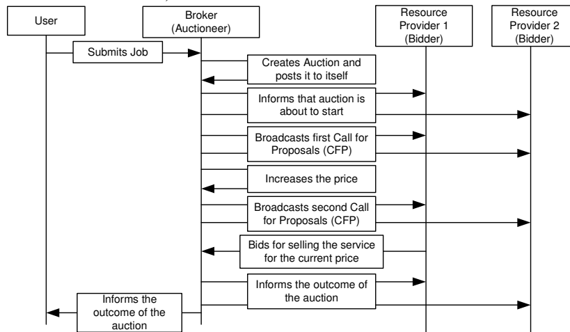
Figure 1. General view of our auction model.
