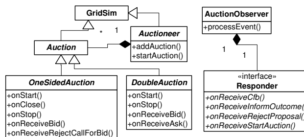
Figure 2. A class diagram of the auction framework.
