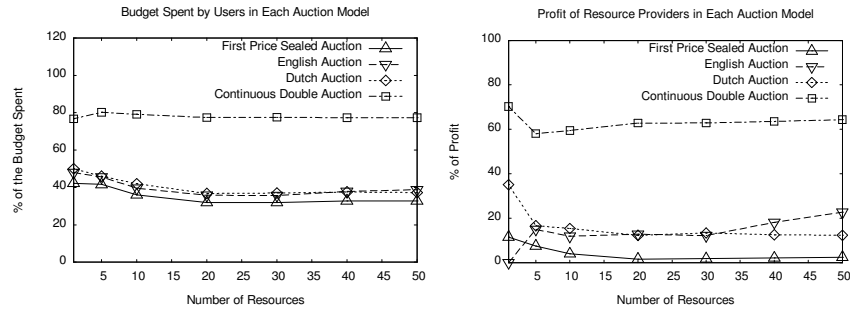
Figure 5. (a) Percentage of aggregated budget spent by users in each auction model. (b) Percentage of aggregated profit made by resource providers.
