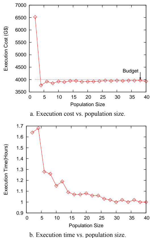
Fig. 16. Execution cost and time for sizes of the population ranged from 2 to 40 when user's budget is G$4000.
