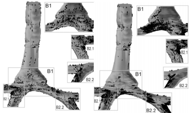
Figure 6 Drug deposition pattern in front and back view of airway with particle diameter in 10µm (left) and 20µm (right). (Square windows are the back view of the bifurcation)
